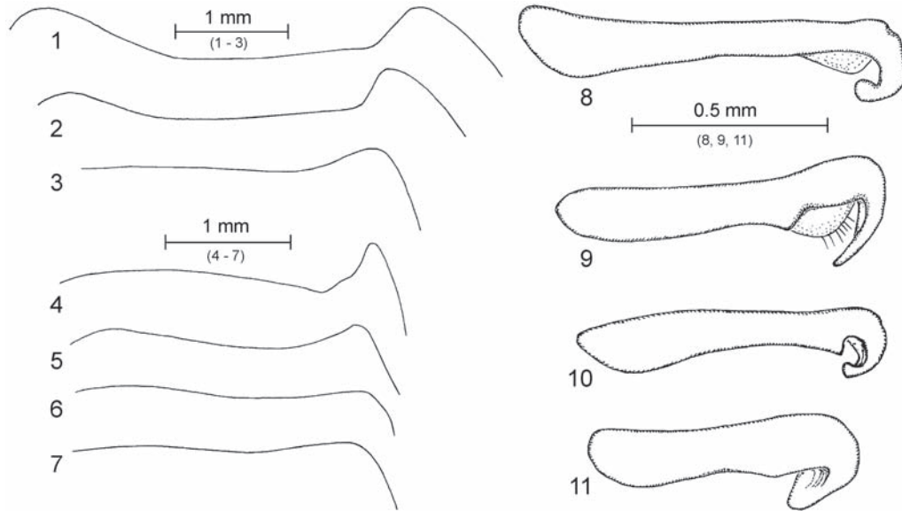
Figs. 1–11: (1–7) Prosternal carina, anterior to the right, venter up. (1) Laccotrephes robustus from Catanduanes, Philippines; (2) L. robustus from Palawan, Philippines; (3) L. pfeifferiae from Perak, West Malaysia; (4) Laccotrephes griseus ; (5) L. longicaudatus sp.n.; (6) L. simulatus from China; (7) L. simulatus from Luzon, Philippines. (8–11) Right parameres, lateral view. (8) L. griseus ; (9) L. longicaudatus sp.n.; (10) L. maculatus , holotype (not on scale); (11) L. simulatus .
